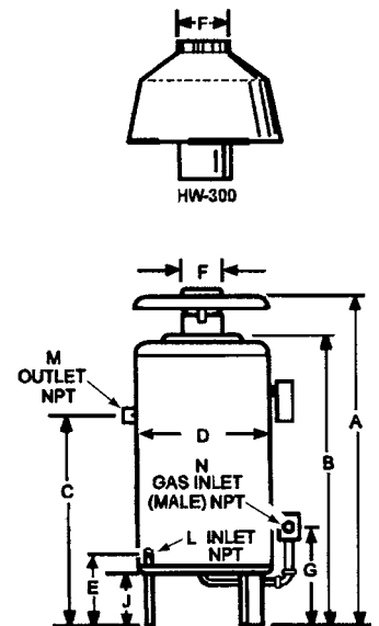
FIGURE 1. DIMENSIONS
