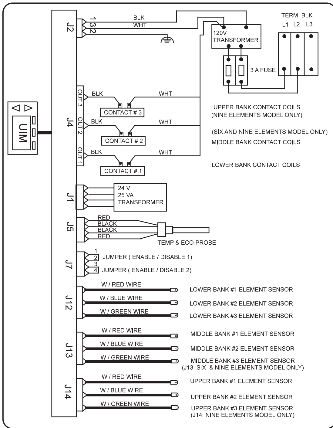
CONTROL CIRCUIT DIAGRAM "Y" CONNECTIONS - ELECTRONIC CONTROL MODELS
