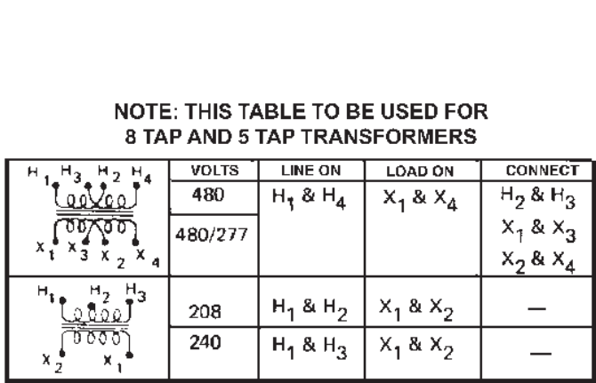
FIGURE 6. - 120 VAC CONTROL CIRCUIT TRANSFORMER CONNECTIONS - ELECTRONIC CONTROL MODELS
